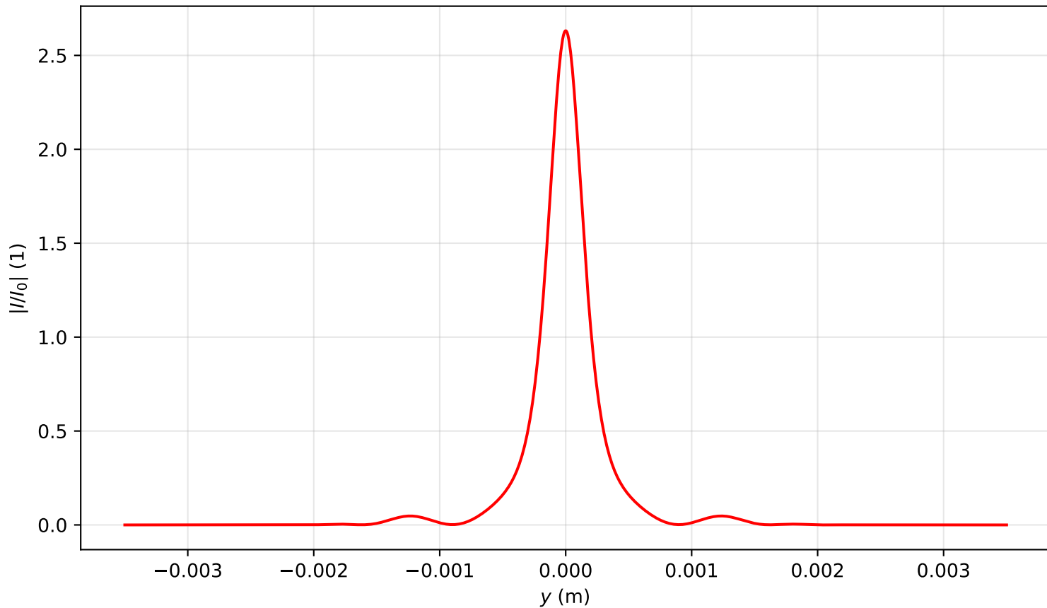
Intensity profile I(x=0, y, z=2.149)/I_0 , \text{Pin}=2.0\text{Pcr} , artificial time
